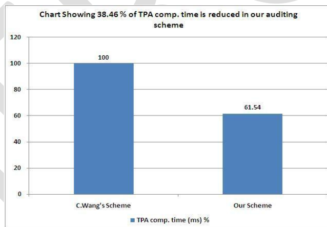
Fig 1.2 Chart Comparisons for TPA Computation Time In %
