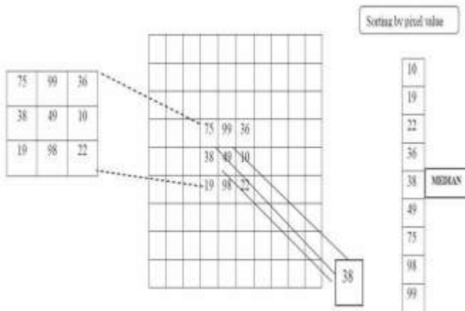
Fig3. Working principle of median filter
