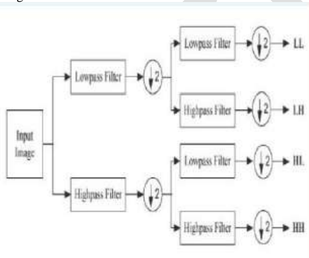
Fig.4 Block diagram of Discrete Wavelet transform
