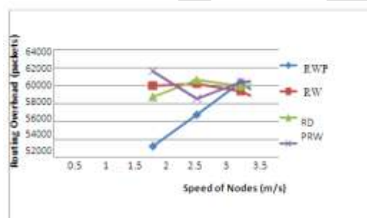
Fig 1 Routing Overhead vs. Speed of Nodes
