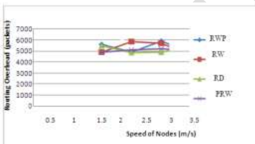
Fig 6 Routing Overhead vs. Speed of Nodes
