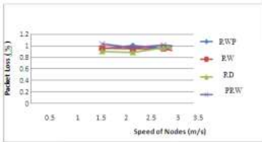
Fig 10 Packet Loss vs Speed of Nodes
