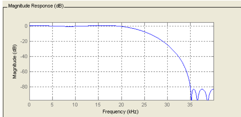
Fig: 5: Magnitude response of FIR filter
