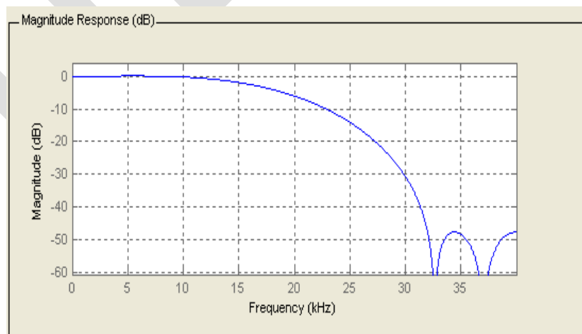
Fig. 8: Magnitude response of Half-band FIR filter
