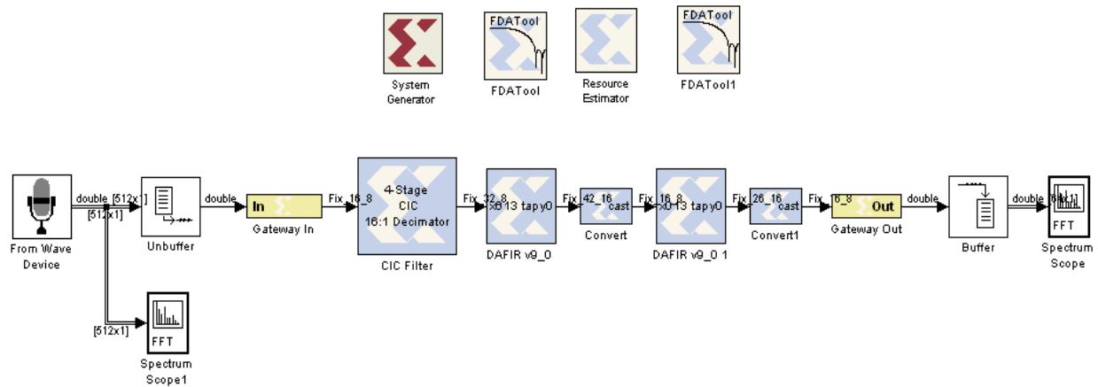
Fig. 7: Simulink model of CIC-Half band FIR-FIR Decimation filter
