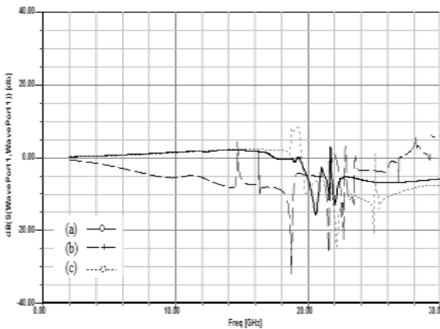
Fig. 4(c) S_{11} Vs Frequency Plot of Second Antenna graph showing parametric variation of Probe length, l inside the LWDRRA (a) l = 3.6\text{mm} , (b) l = 4.2\text{mm} (c) l = 4.8\text{mm}
