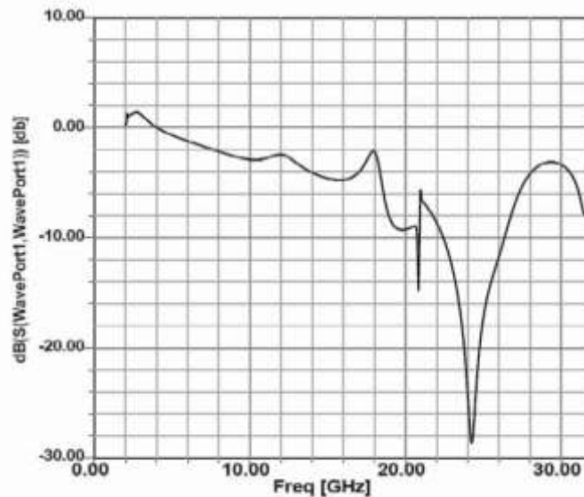
Fig. 3 S_{11} Vs Frequency Plot of Second Antenna
