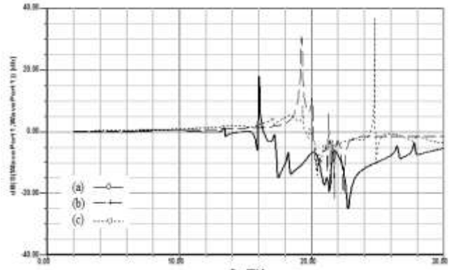
Fig. 4(b) S_{11} Vs Frequency Plot of Second Antenna graph showing parametric variation of Probe length, l inside the LWDRRA (a) l = 1.8\text{mm} , (b) l = 2.4\text{mm} (c) l = 3.0\text{mm}
