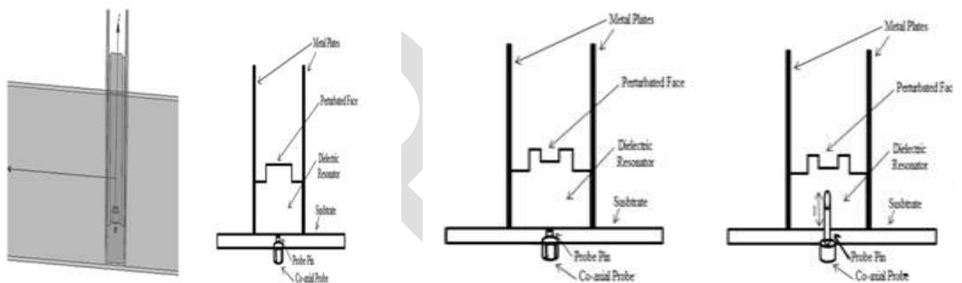
Figure 1(a) LWRDRA Designed & Simulated on HFSS 3D view, (b) First Antenna Designed, (c) Second Antenna Design and (d) Second Antenna Design, with probe pin, l set as project variable for parametric study of Antenna
