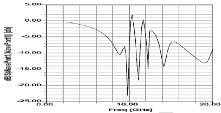
Fig. 2 S_{11} Vs Frequency Plot of First Antenna
